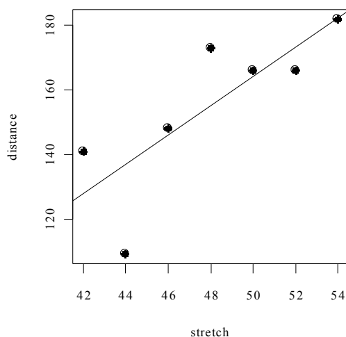
Figure 18: Plot of distance versus stretch for the elastic band data, with fitted least squares line
