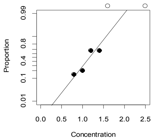
Figure 26: Plot, versus concentration, of \log(\text{odds}) [= \text{logit}(\text{proportion}) ] of patients not moving. The line is the estimate of the proportion of moves, based on the fitted logit model.
