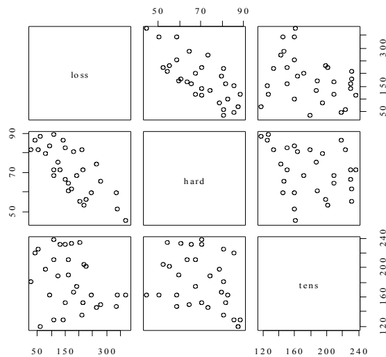
Figure 20: Scatterplot matrix for the Rubber data frame from the MASS package.
